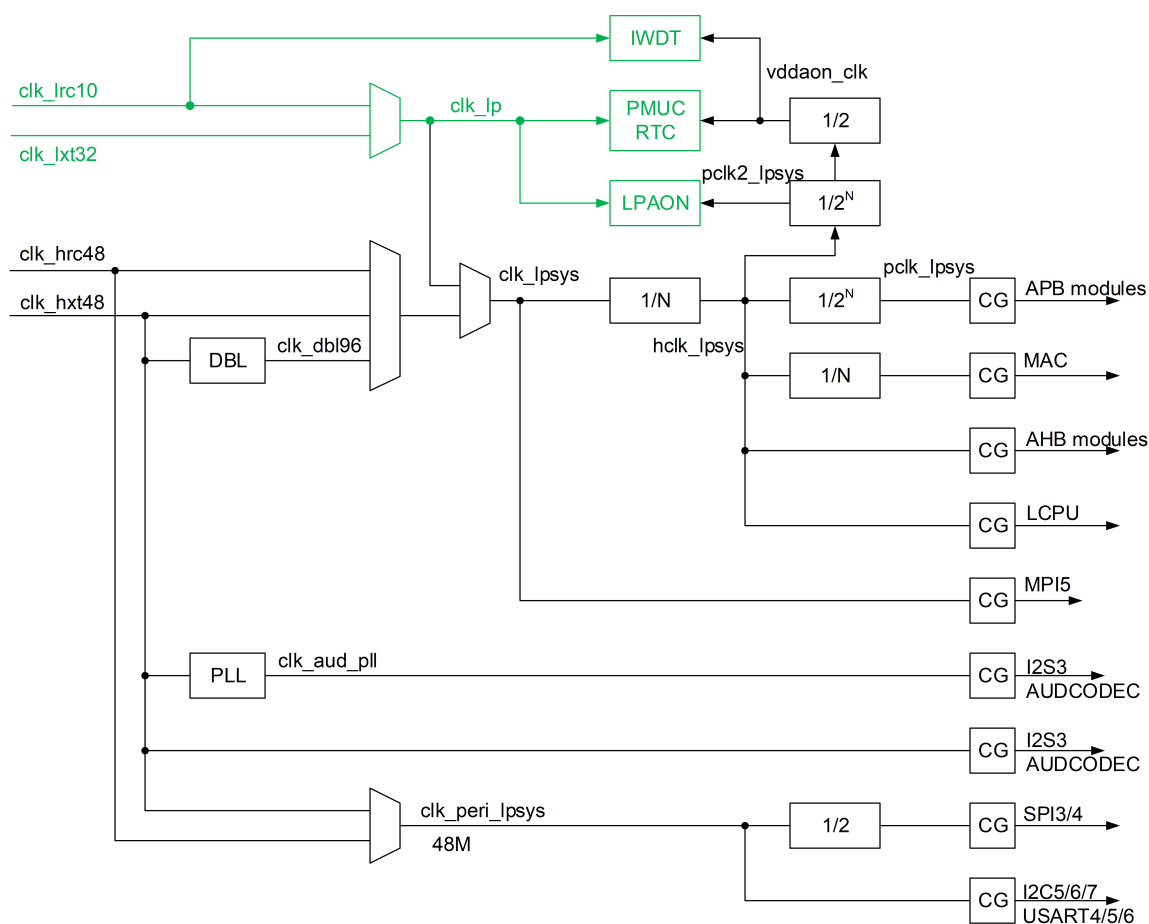
Figure 2-2: LPSYS Clock Structure
