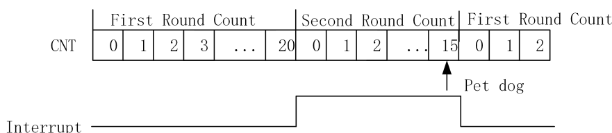
Figure 9-18: Mode 2 The effect of the 'dog feeding' operation on the counter during the second round of counting is the same as in the first round (assuming the timeout value is 20)
