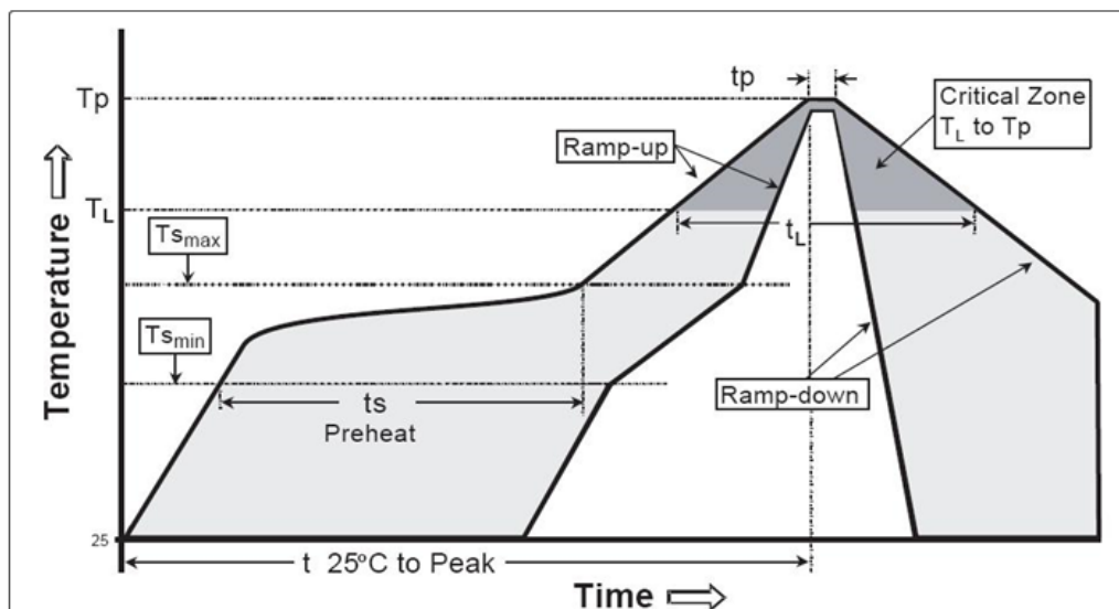
Figure 5-9: Graded Reflow Soldering
