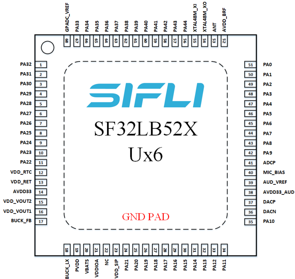
Figure 5-1: SF32LB52X pinout diagram
