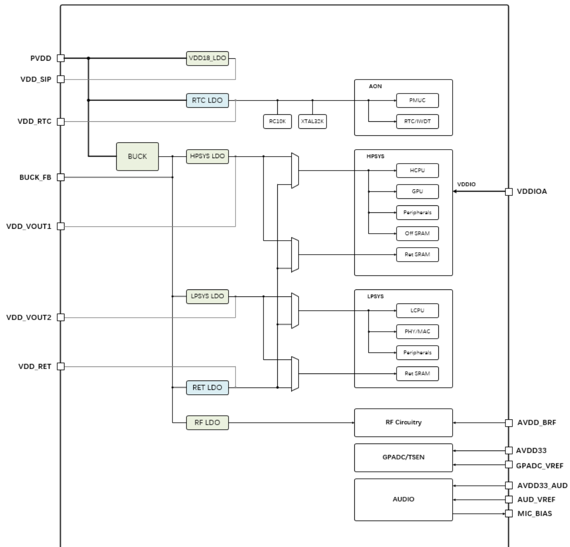
Figure 1-3: Power Management Architecture of QFN Package
