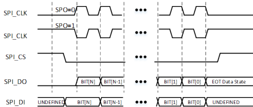
Figure 3-7: SPI Sequence at SPH=1
