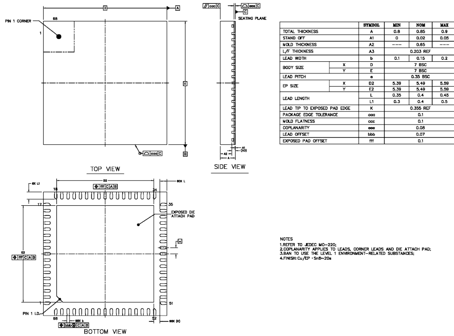
Figure 5-2: QFN68L Package Dimensions
