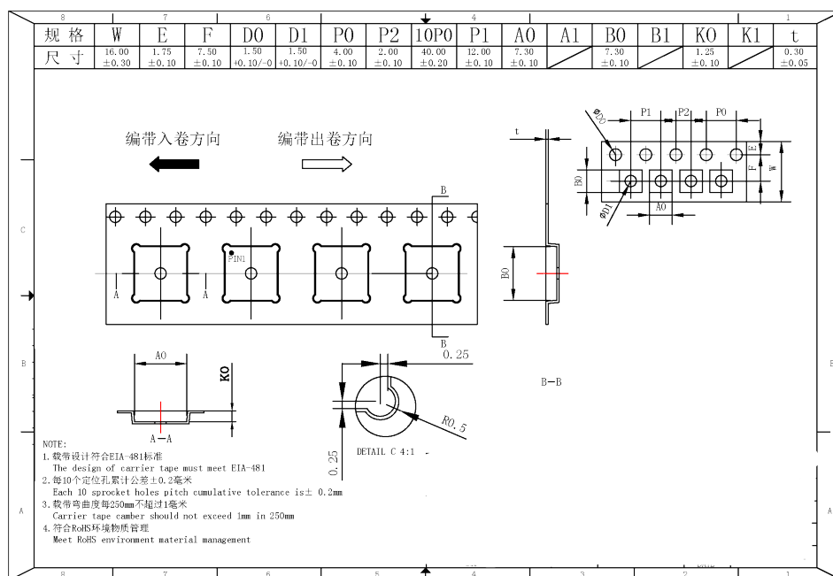
图 5-3: 载带尺寸
