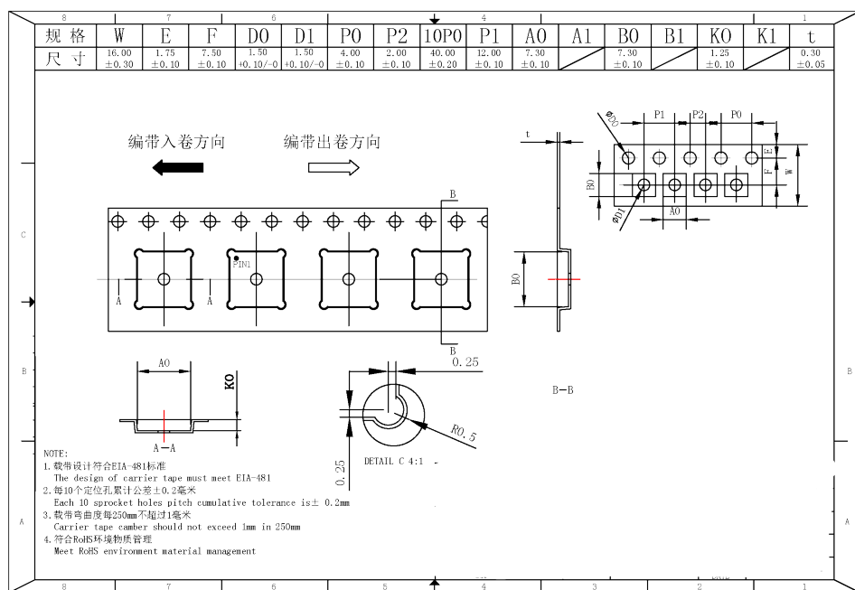
图 5-3: 载带尺寸
