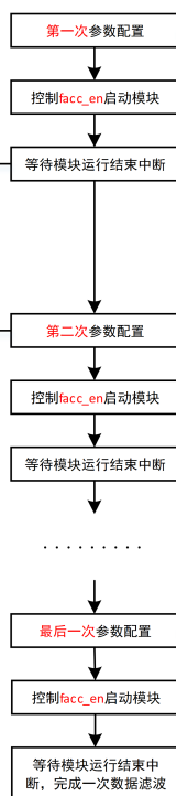
Figure 12-1: configuration Procedure Flowchart in Non-Cache Mode
