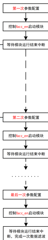
Figure 12-2: Flowchart of the configuration Procedure in Cache Mode
