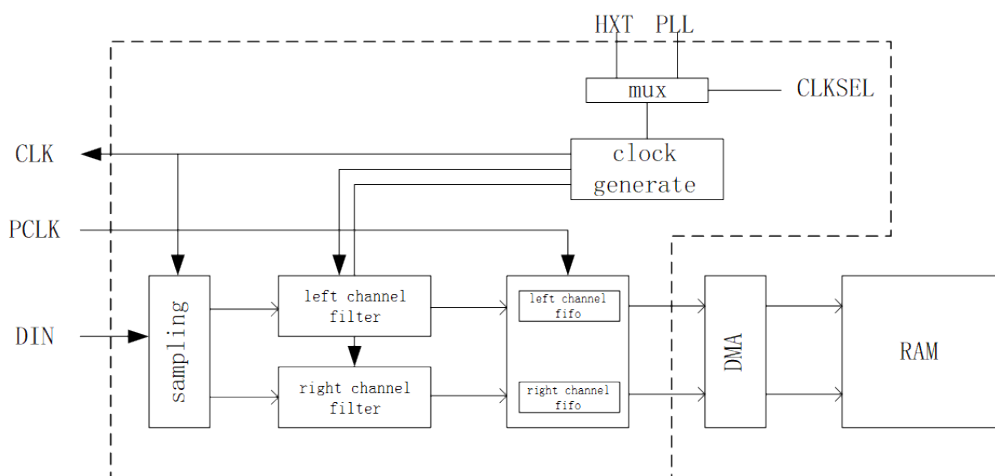
Figure 11-2: Overall Structure of the PDM Module
