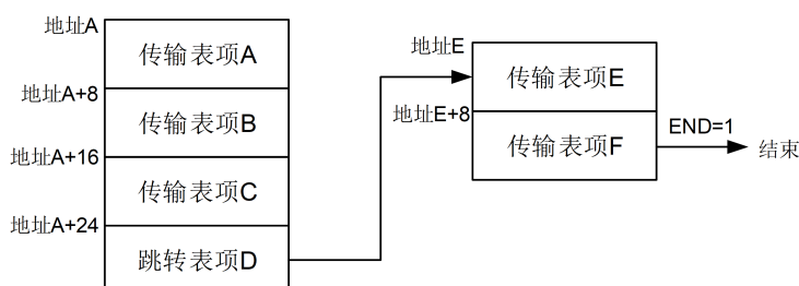
Figure 14-2: Example of an ADMA chain descriptor table
