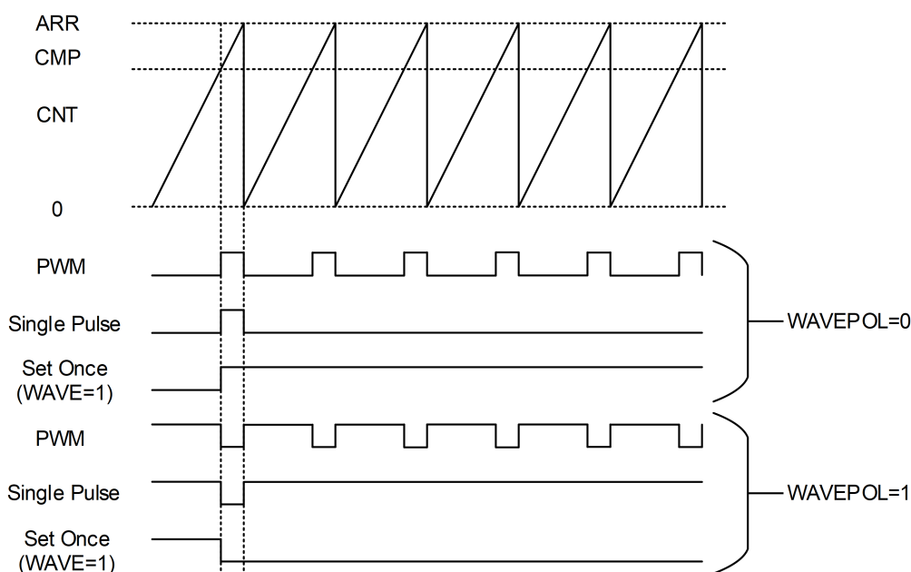
Figure 9-14: PWM Output
