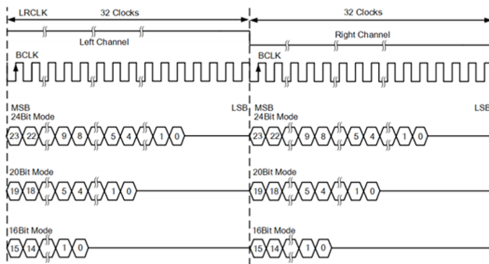
Figure 11-5: I2S 左对齐
