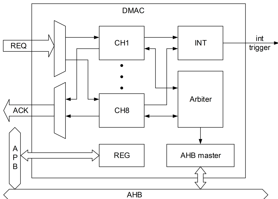
Figure 6-1: DMAC 结构图
