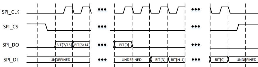
Figure 7-8: Microwire 协议单次通信时序
