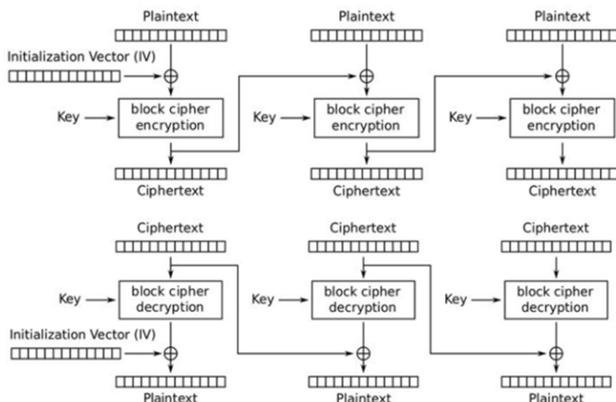
Figure 13-3: CBC 模式解密
