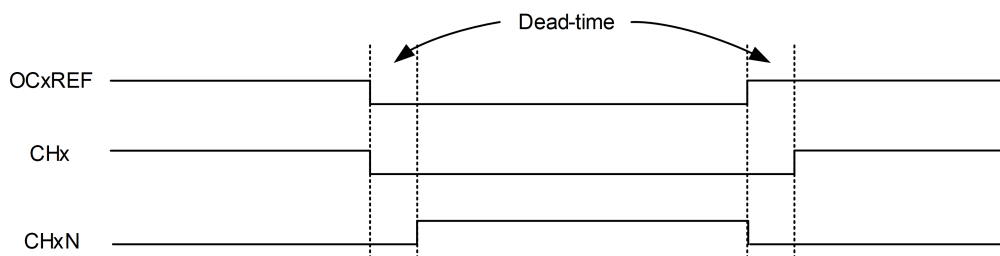
Figure 9-6: 带死区的互补 PWM 输出
