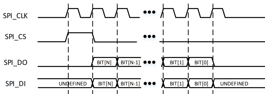
Figure 7-6: TI-SSP 协议通信时序
