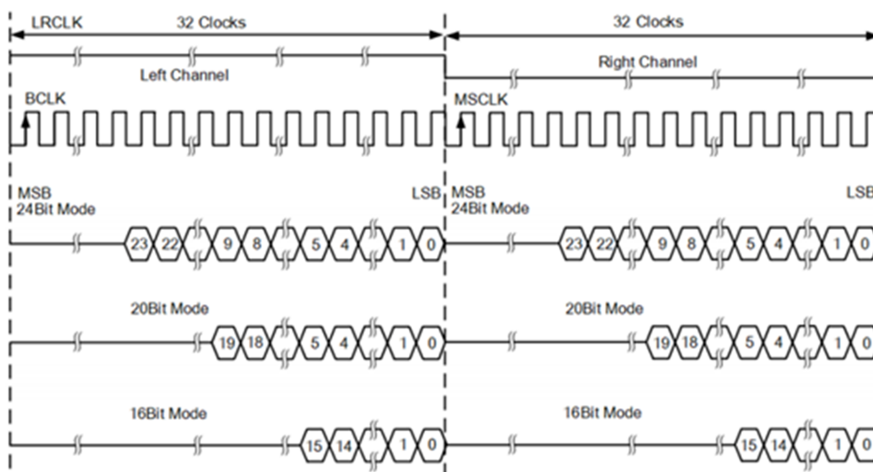
Figure 11-6: I2S 右对齐
