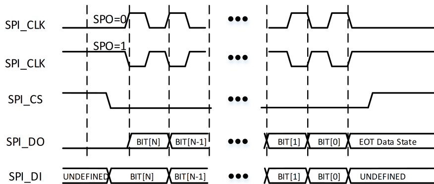
Figure 7-5: SPI 协议连续传输时序
