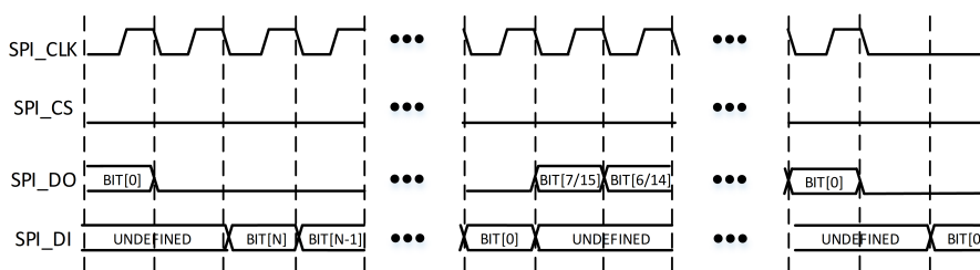
Figure 7-9: Microwire 协议连续传输时序
