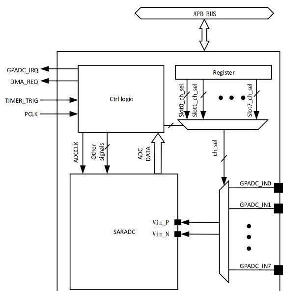
Figure 8-1: GPADC 框图
