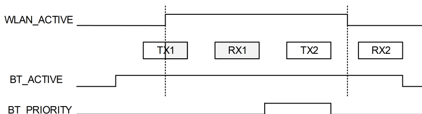
Figure 15-3: WLAN_ACTIVE 影响示例
