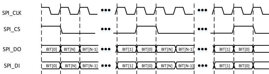
Figure 7-7: TI-SSP 协议连续通信时序
