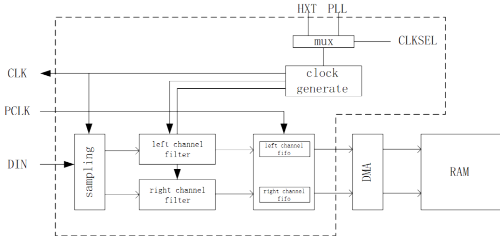
Figure 11-2: PDM 模块的整体结构
