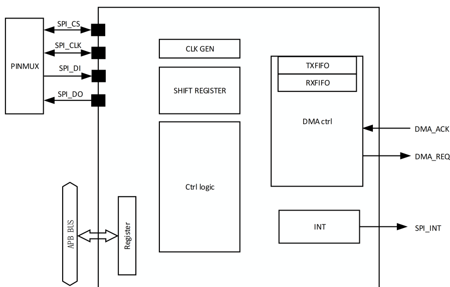
Figure 7-2: SPI 结构图
