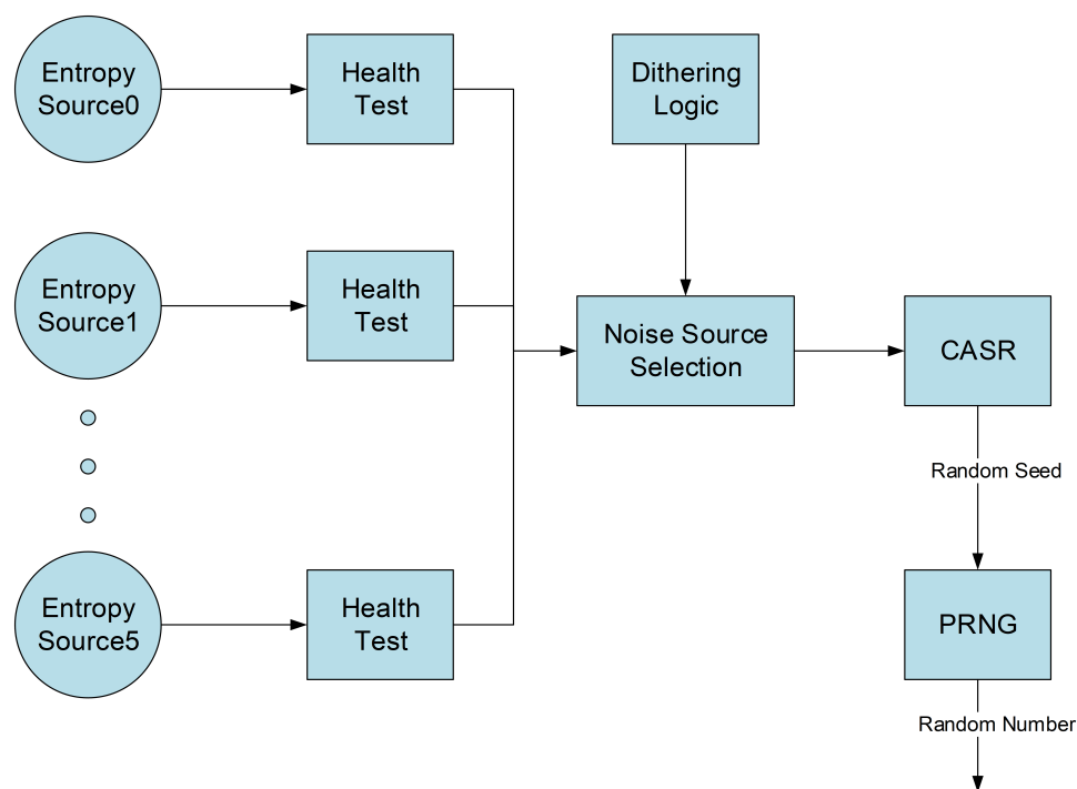
Figure 13-4: TRNG 结构图
