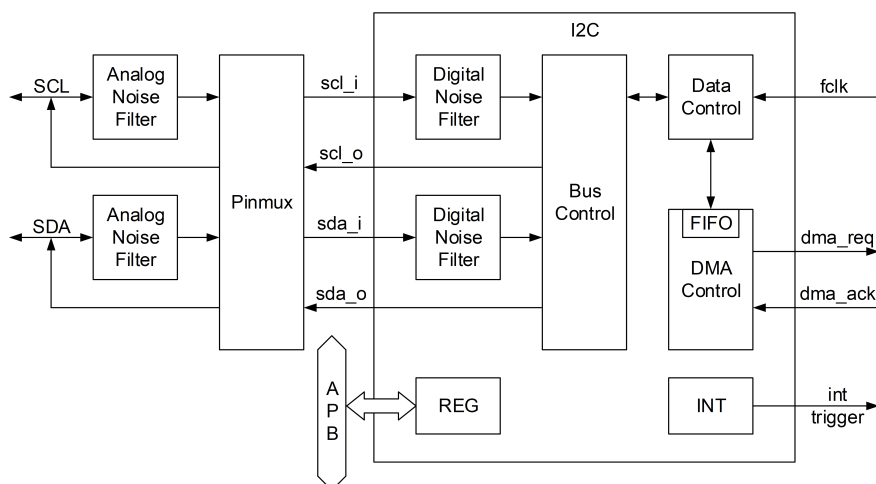
Figure 7-1: I2C 结构图
