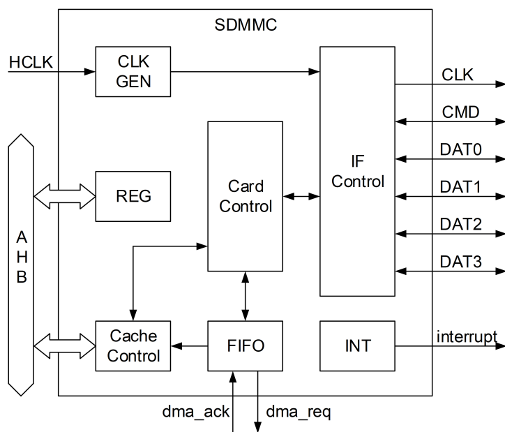
Figure 14-3: SDMMC 结构图
