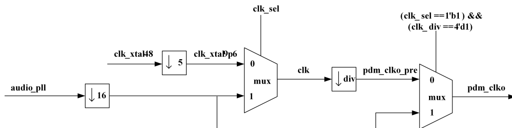
Figure 11-3: PDM 模块的时钟结构
