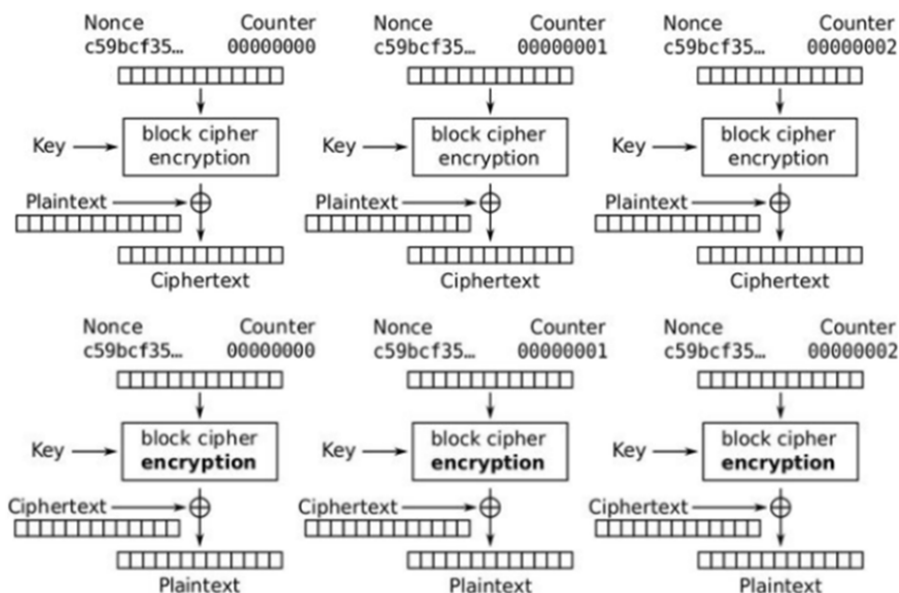
Figure 13-2: CTR 模式解密
