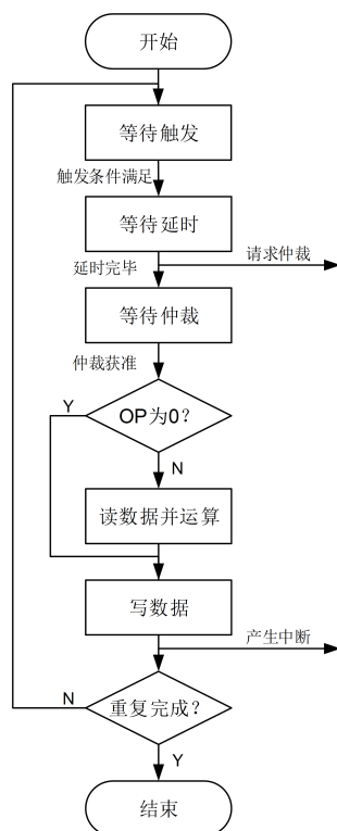
Figure 7-11: PTC 通道执行流程图
