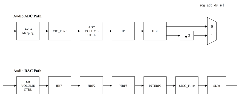
Figure 11-8: Audcodec 通路架构图
