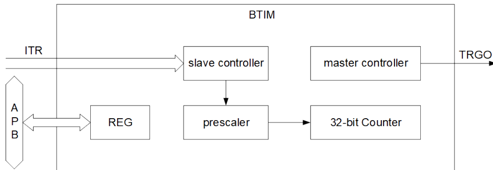
Figure 9-1: BTIM Block Diagram
