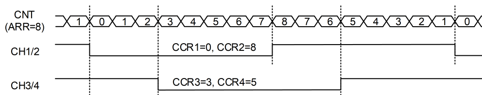
Figure 9-5: Asymmetric PWM output
