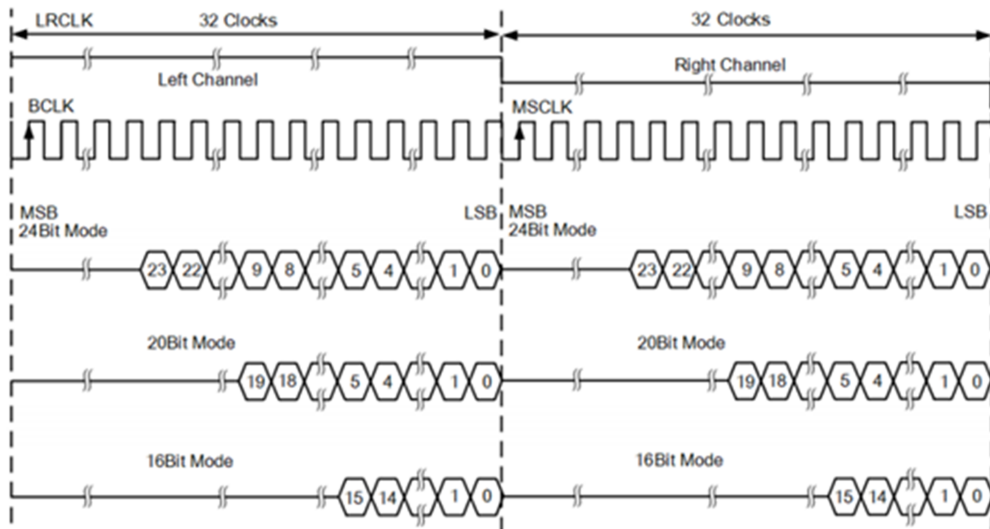
Figure 11-6: I2S Right-aligned
