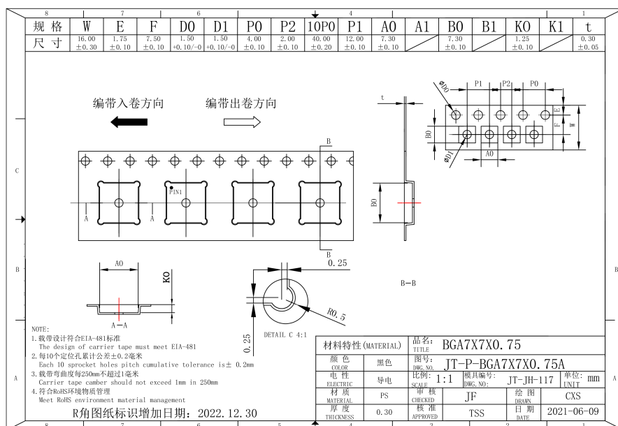
图 5-3: 载带尺寸
